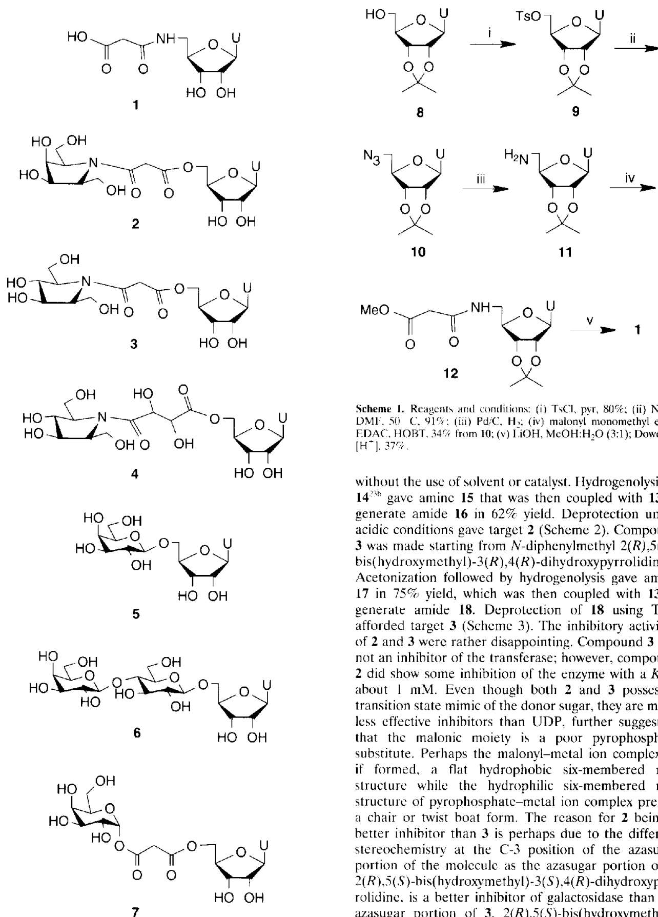
Figure 5. Structures of target compounds 1–7 .
