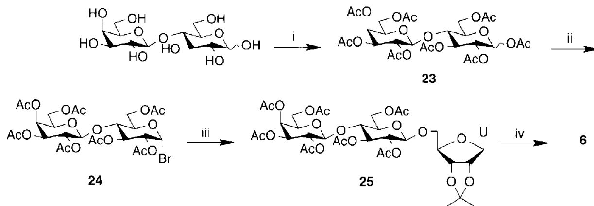
Scheme 6. Reagents and conditions: (i) acetic anhydride, pyr., 92%; (ii) hydrogen bromide in acetic acid (30%), \text{CH}_2\text{Cl}_2 ; (iii) 8 , \text{Hg}(\text{CN})_2 , \text{CH}_2\text{Cl}_2 , 35 °C, 65%; (iv) \text{NaOMe} , \text{MeOH} : Dowex 50 [ \text{H}^+ ], 43%.
