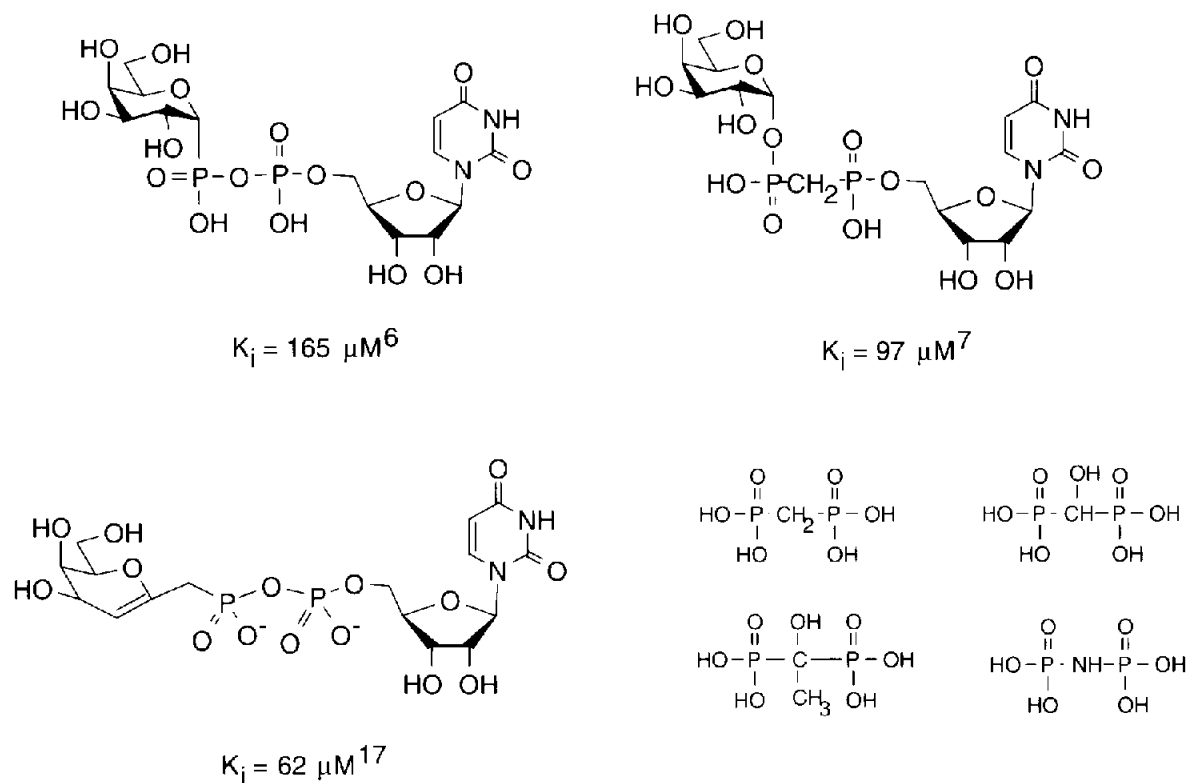
Figure 2. Galactosyltransferase inhibitors containing modified pyrophosphate groups.
