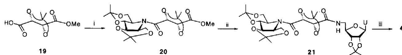
Scheme 4. Reagents and conditions: (i) 17, EDAC, DMAP, 84%; (ii) KOH, MeOH; 11, EDAC, DMAP, 41%; (iii) \text{TFA}:\text{H}_2\text{O} (9:1), 17%.
