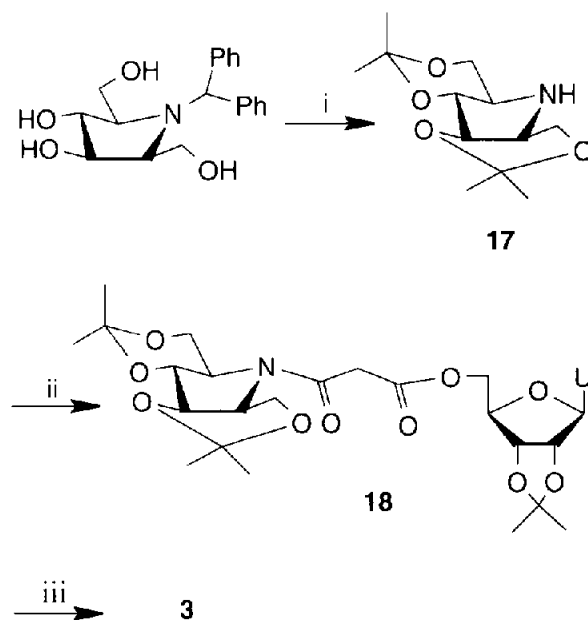
Scheme 3. Reagents and conditions: (i) methoxypropene, \text{CH}_2\text{Cl}_2 -THF, p -TsOH; \text{Pd}(\text{OH})_2 , 50 psi, \text{H}_2 , 75%; (ii) 13, EDAC, DMAP, \text{CH}_2\text{Cl}_2 , 76%; (iii) \text{TFA}:\text{H}_2\text{O} (9:1), 75%.
