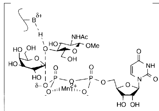
Figure 3. Proposed transition state of the galactosyltransferase reaction.
