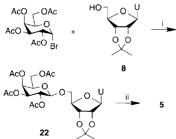
Scheme 5. Reagents and conditions: (i) \text{Hg}(\text{CN})_2 , \text{CH}_2\text{Cl}_2 , 35 °C, 66%; (ii) \text{NaOMe} , \text{MeOH} : \text{AcOH} : \text{HCl} (3:1), 95%.
