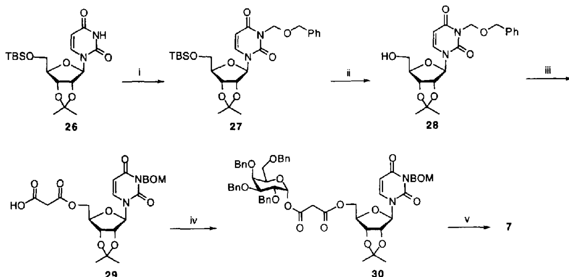
Scheme 7. Reagents and conditions: (i) BOMCl, i -Pr 3 NEt, CH 2 Cl 2 , 0 °C, 89%; (ii) Bu 4 NF, THF, 94%; (iii) Meldrum's acid, 100 °C, 77%; (iv) 2,3,4,6-tetra-benzyl galactosylpyranose β-imidate, CH 2 Cl 2 , -20 °C, 52%; (v) Pd(OH) 2 , H 2 , EtOH, CHCl 3 , H 2 O, 44%.
