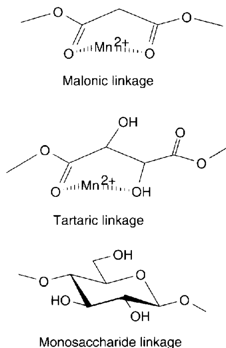
Figure 4. Designed mimics of pyrophosphate- \text{Mn}^{2+} complex.
