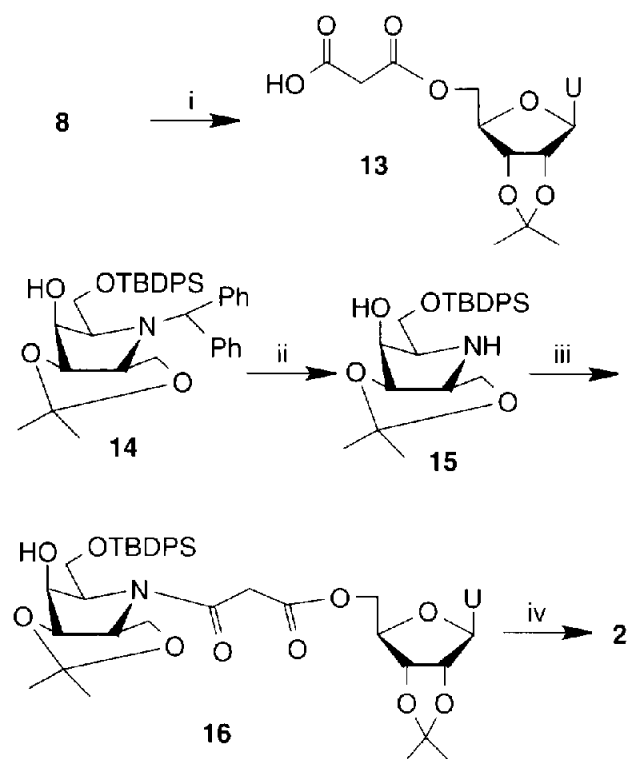
Scheme 2. Reagents and conditions: (i) Meldrum's acid, 66%; (ii) \text{Pd}(\text{OH})_2 , \text{H}_2 , 50 psi; (iii) 13, EDAC, HOBT, 62% from 14; (iv) \text{TFA}:\text{H}_2\text{O} (9:1), 44%.
