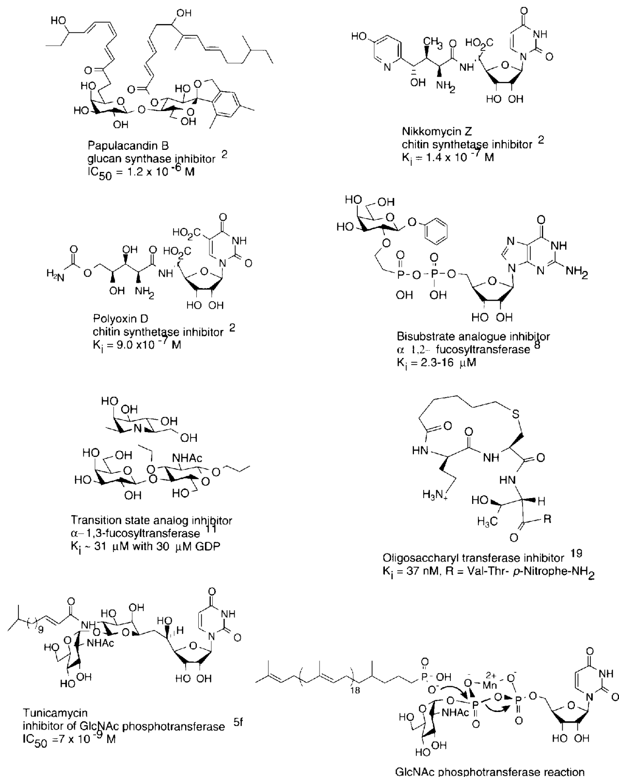
Figure 1. Examples of glycosyltransferase inhibitors. Tunicamycin appears to mimic the transition state of the GlcNAc phosphotransferase reaction.
